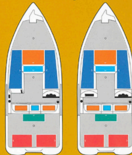
■ Dry Storage ■ Batteries & Gas Tanks ■ Live Wells ■ Rod Box ■ Ice Chest
